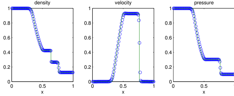
Fig. 1. Interface-sharpener result for the Sod shock tube problem at time t = 0.15 using a 100 grid. The solid line shown in the graph is the exact solution.
