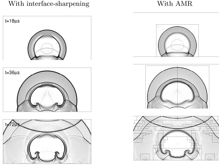
Fig. 5. Numerical results for a blast wave problem in two dimensions. Schlieren images of density are shown at three different times t = 18, 36, 72 \mu s obtained using the methods with anti-diffusion (the left column) and with local adaptive mesh refinement (the right column).
