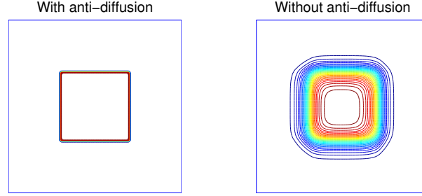
Fig. 3. Numerical results for a passive evolution of a square column. Contours of the density are shown at time t = 0.02\text{s} obtained using the method with and without interface-sharpening on a 100 \times 100 grid.
