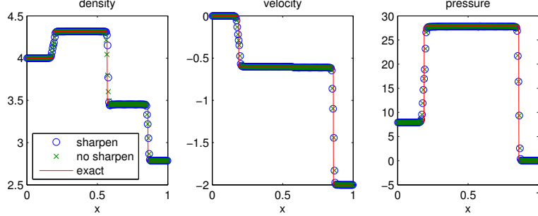
Fig. 2. Interface-sharpener result for the aluminum impact problem at time t = 50 \mu\text{s} using 200 grids. The solid line shown in the graph is the exact solution and the symbol “x” is the result obtained using the method without interface-sharpener.
