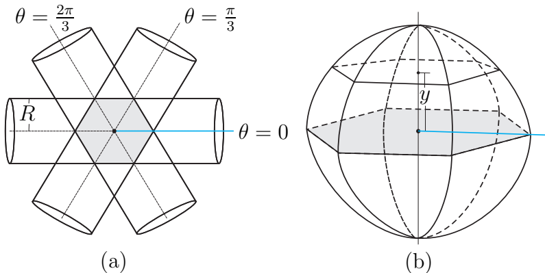
Figure 1: Intersection of three cylinders. (a) Vertical view. (b) The solid.
